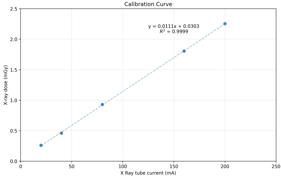
Figure 1: Calibration Curve
